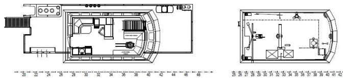
Bridge deck
